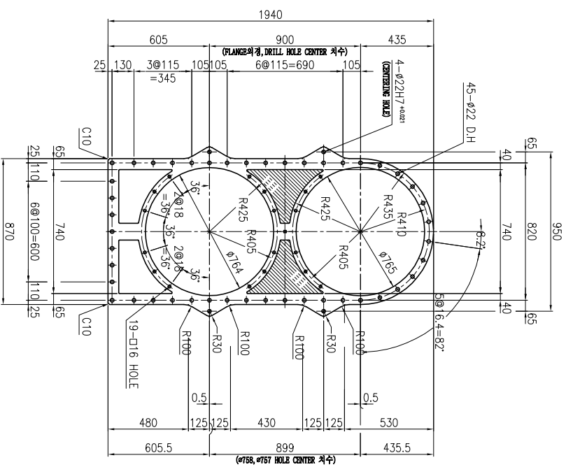
VIEW "B-B" (TAIL SIDE)
