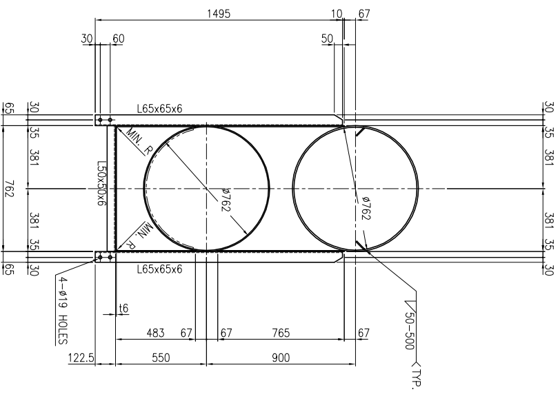
SECTION "F-F"
